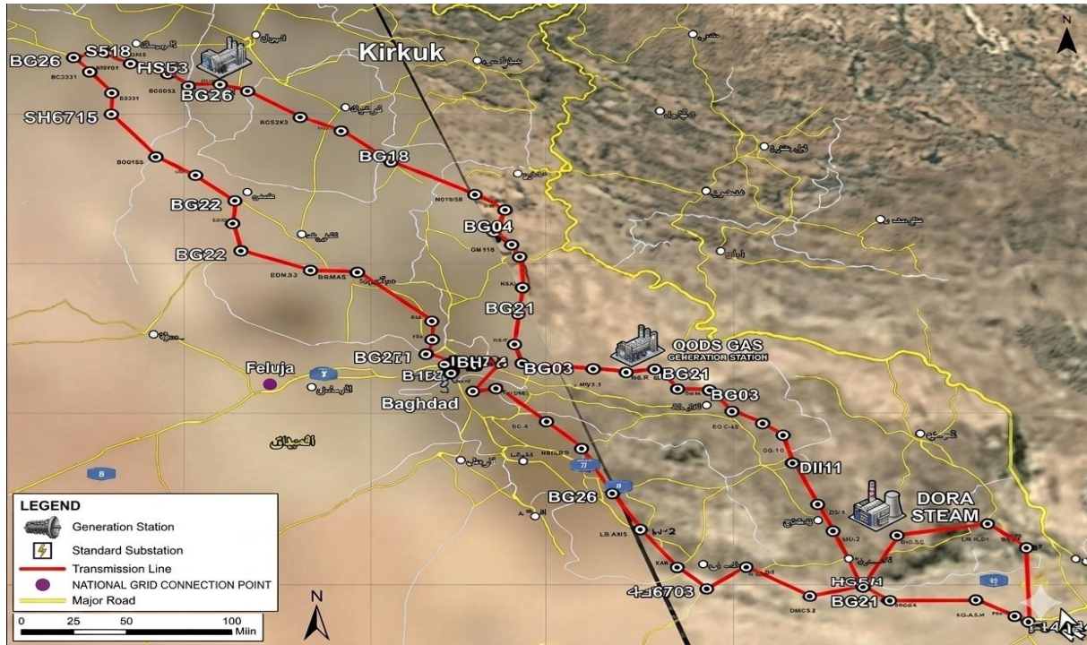
Fig. 13. The best paths of a MT-HVDC proposed for the Iraqi grid [18].
