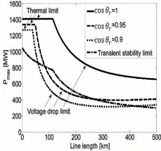
Fig. 2. Characteristics of AC lines loadability with different power factor values [18], [19].
