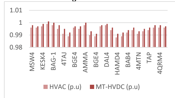
Fig. 11. ISHVG voltage profile under 10% operating conditions.
