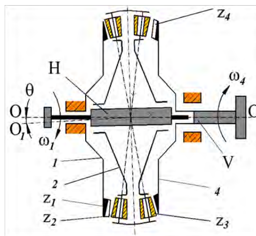
Figure 4. 2K-H kinematic scheme
