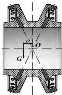
Figure 1. Satellite block imbalance
