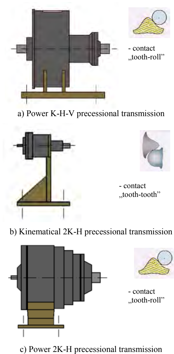
Figure 6. Researched precessional gearbox
